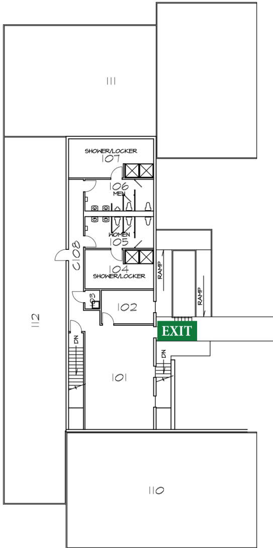
NORTH FIRST FLOOR PLAN 0 8 16 24 32 FEET
